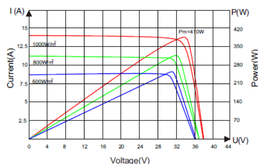
I-V křivka panelu (SPV410-R54DWML)
